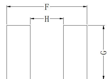
推荐焊盘尺寸 Recommend PC Board Pattern
